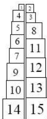
Figure 1: A possible stacking of n = 15 blocks.
