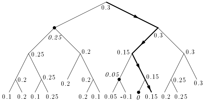
Figure 4: A search path in T .
